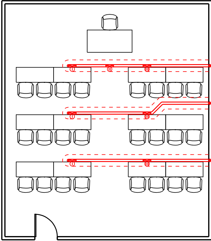
Layout Option 1
